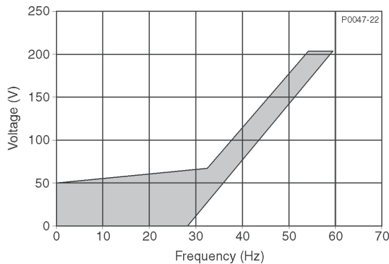
Figure 2 - AVC63-4/4D Frequency Compensation Characteristic 60 Hz
