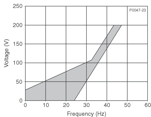
Figure 3 - AVC63-4/4D Frequency Compensation Characteristic 50 Hz
