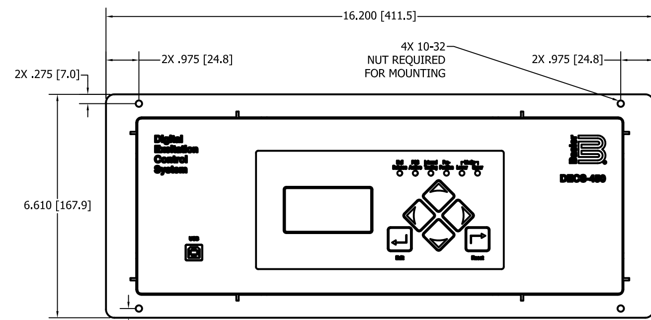
ESCUTCHEON PLATE
