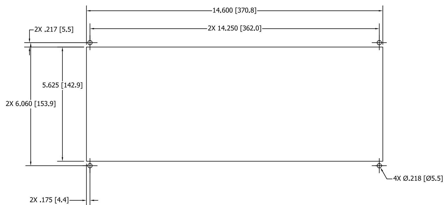
PANEL CUTTING AND DRILLING FOR ESCUTCHEON MOUNTING
