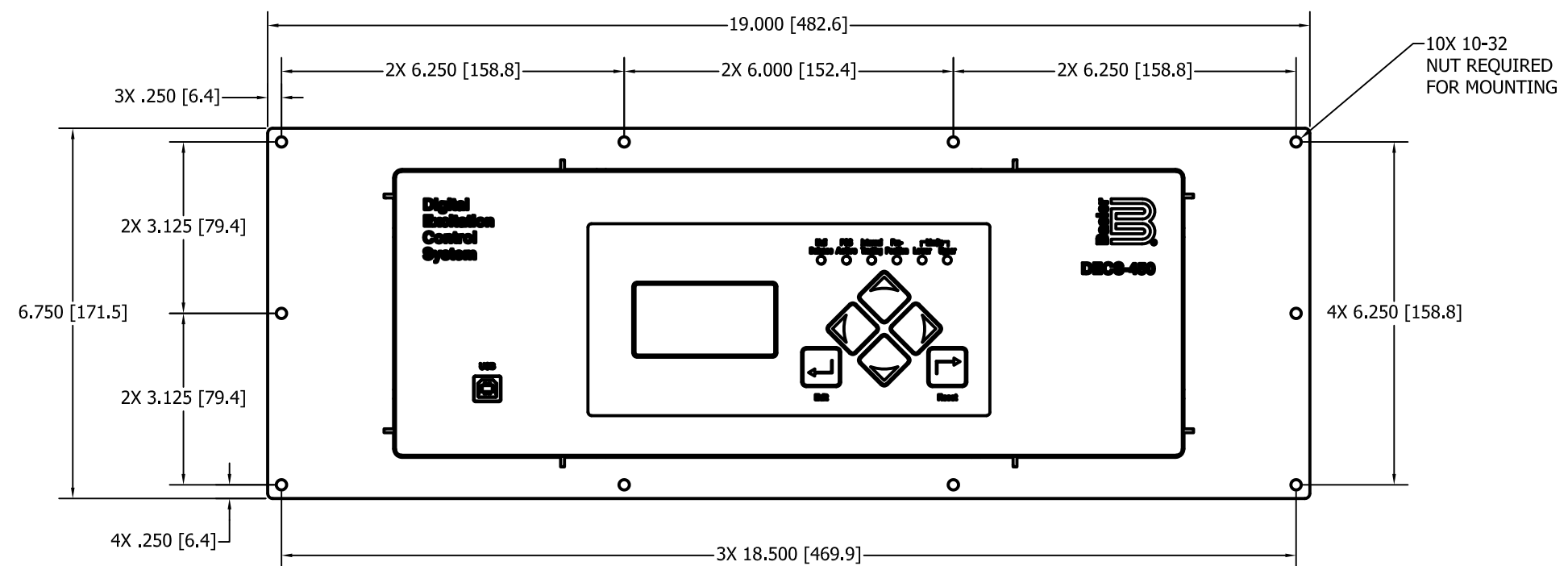
DECS-300 CONVERSION
